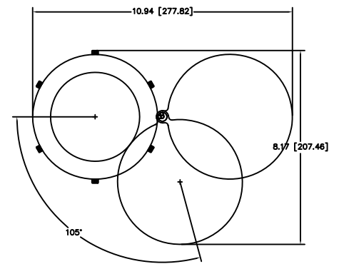
MINIMUM SHUTTER SWING CLEARANCE
