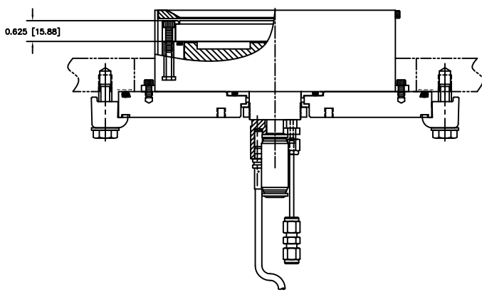
DIRECTLY WATER COOLED TARGET (-2 ASSY)
