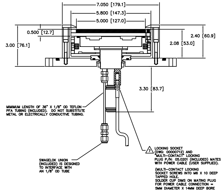
BONDED TARGET ASSEMBLY SHOWN
