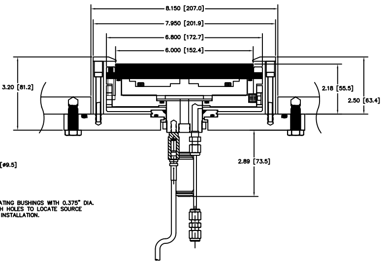
DIRECT WATER COOLED TARGET SHOWN
