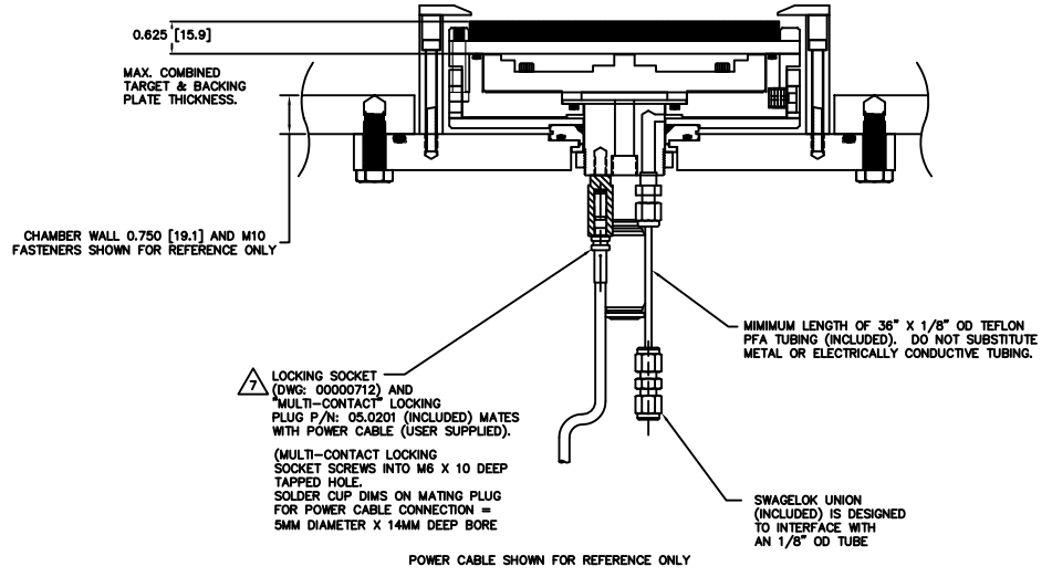
BONDED TARGET ASSEMBLY SHOWN
