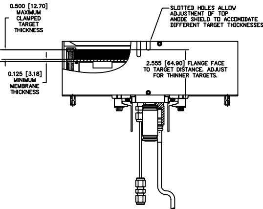
SEMI-PERMANENT MEMBRANE FOR CLAMPED TARGETS (-3 ASSY)
