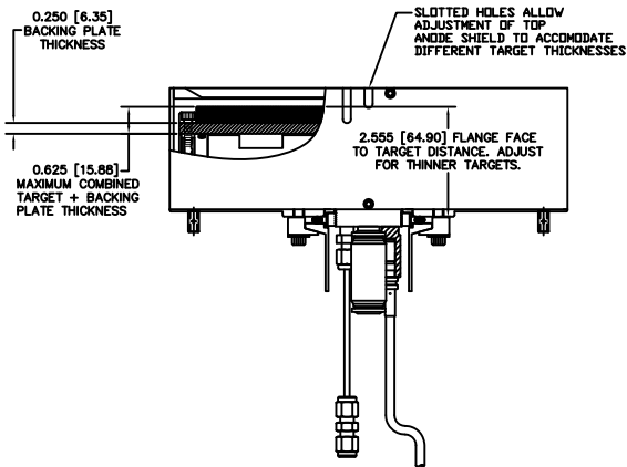
BONDED TARGET ASSEMBLY (-1 ASSY)
