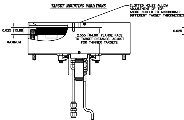
DIRECTLY WATER-COOLED TARGET (-2 ASSY)
