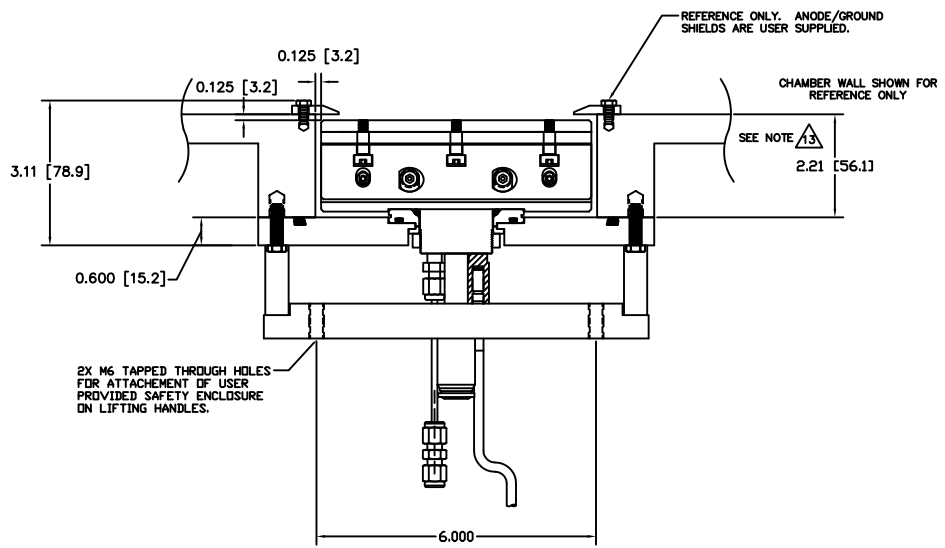
BONDED TARGET ASSEMBLY SHOWN
